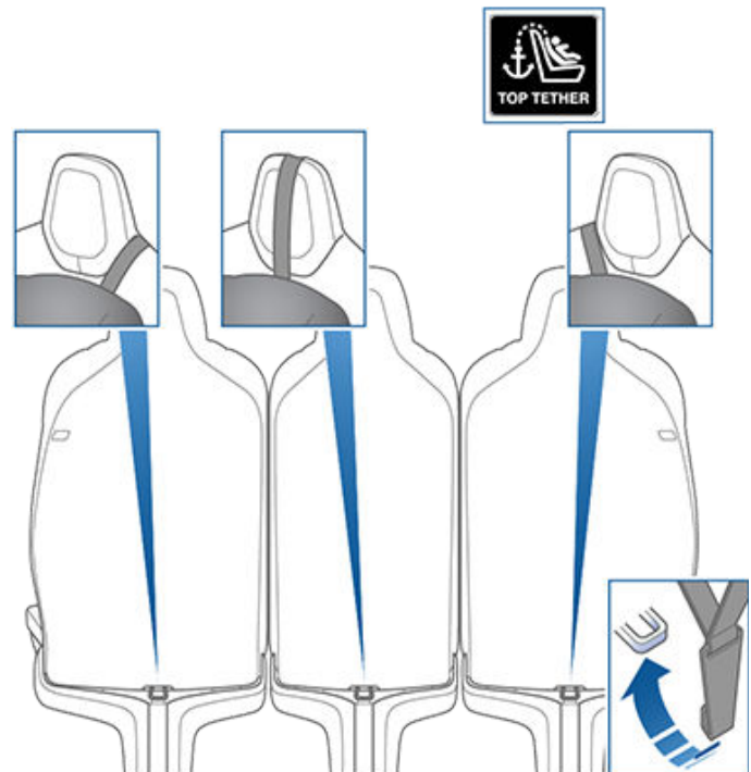
Single Strap - Second Row Bench Seats
